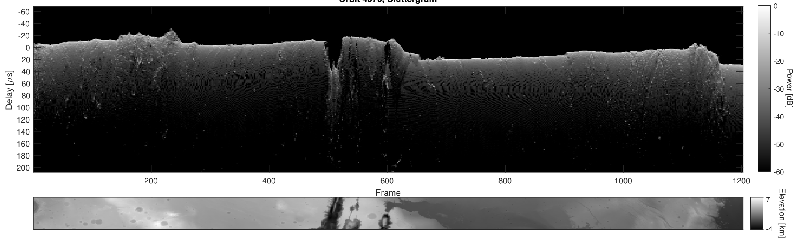
Orbit 4076, Cluttergram
