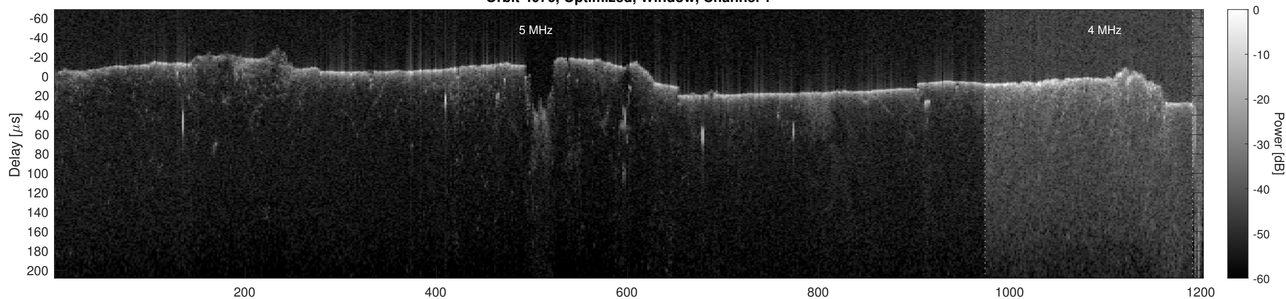
Orbit 4076, Optimized, Window, Channel 2
