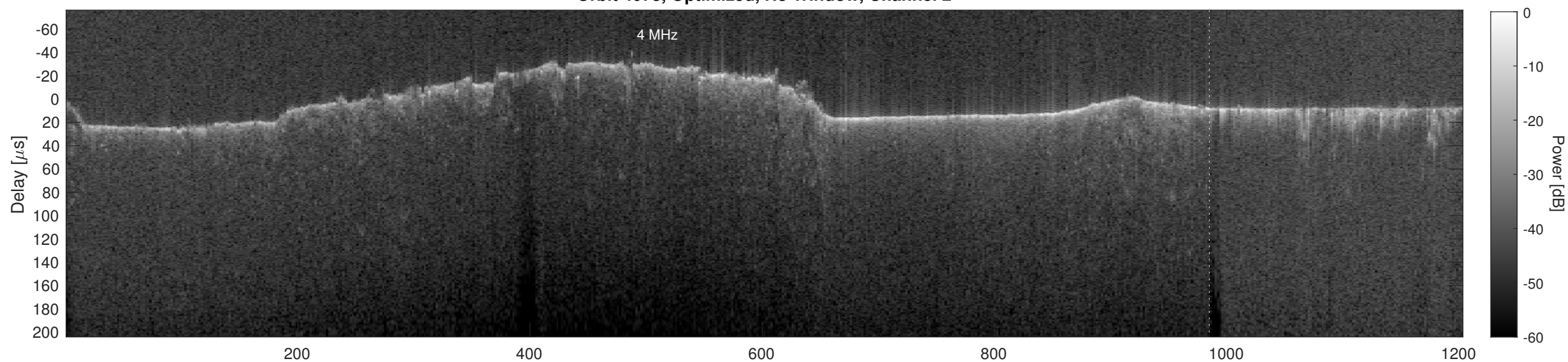
Orbit 4078, Cluttergram
