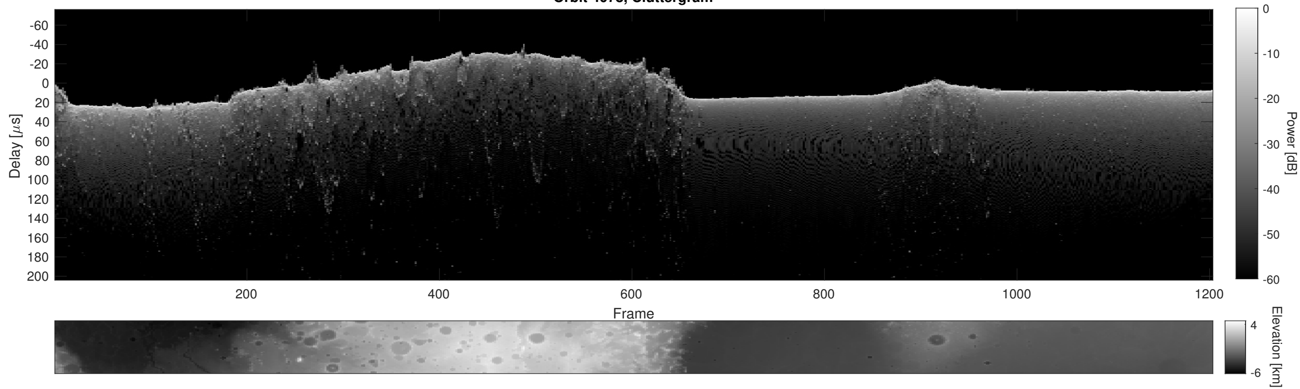
Orbit 4078, Cluttergram
