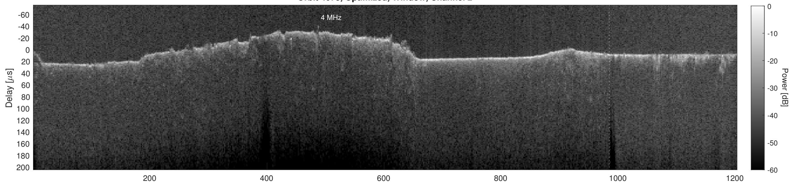
Orbit 4078, Cluttergram
