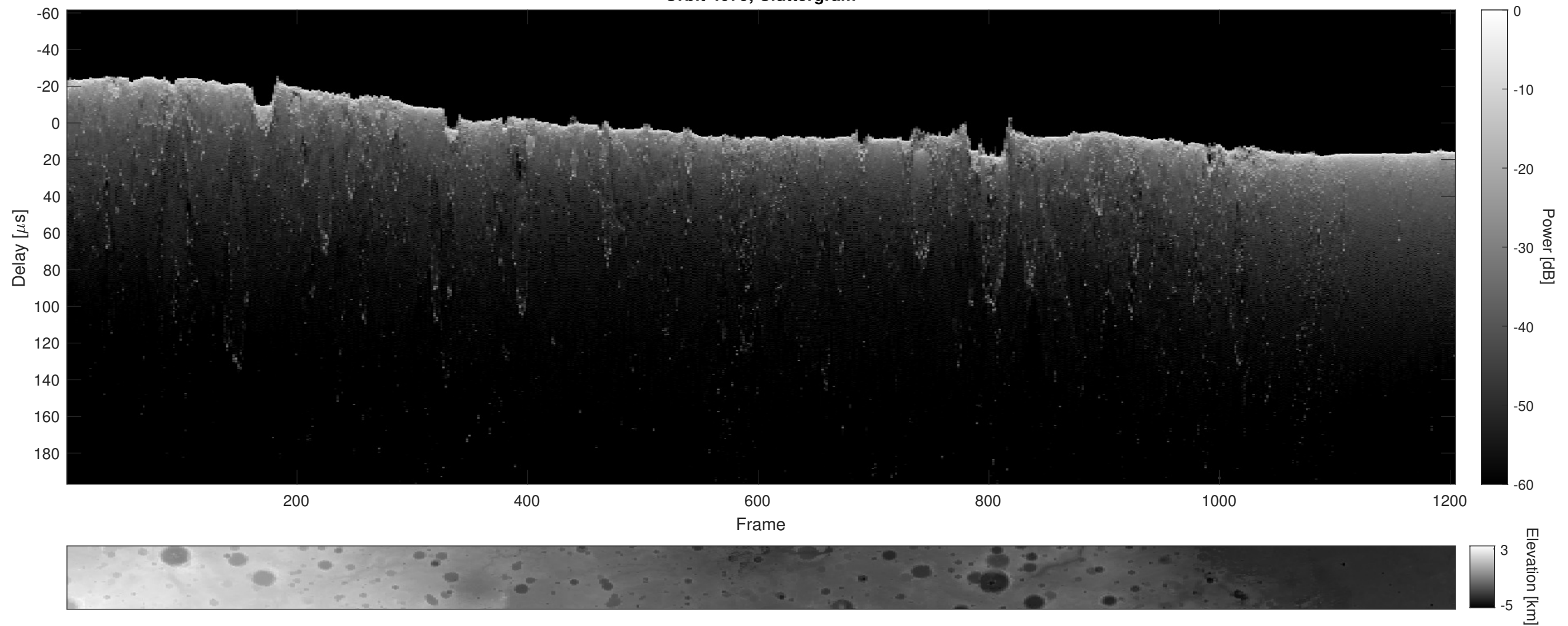
Orbit 4079, Cluttergram
