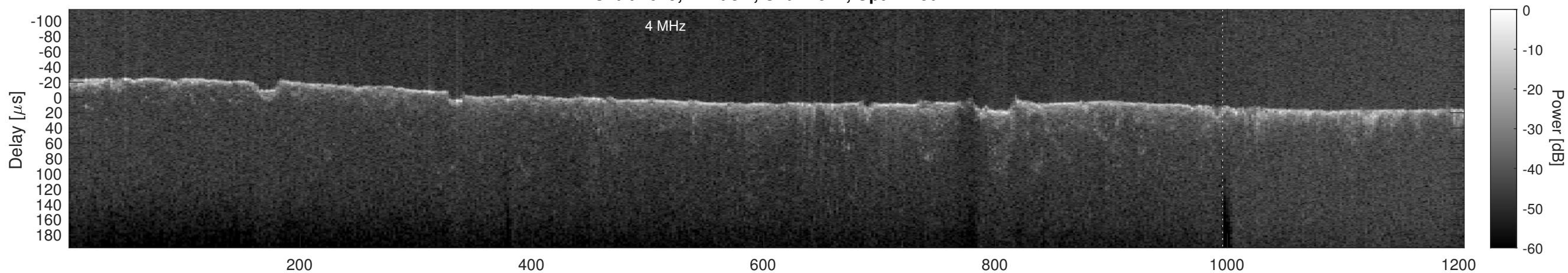
Orbit 4079, Cluttergram
