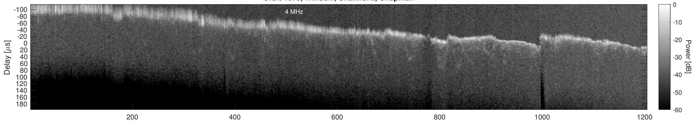
Orbit 4079, Window, Channel 2, Optimized
