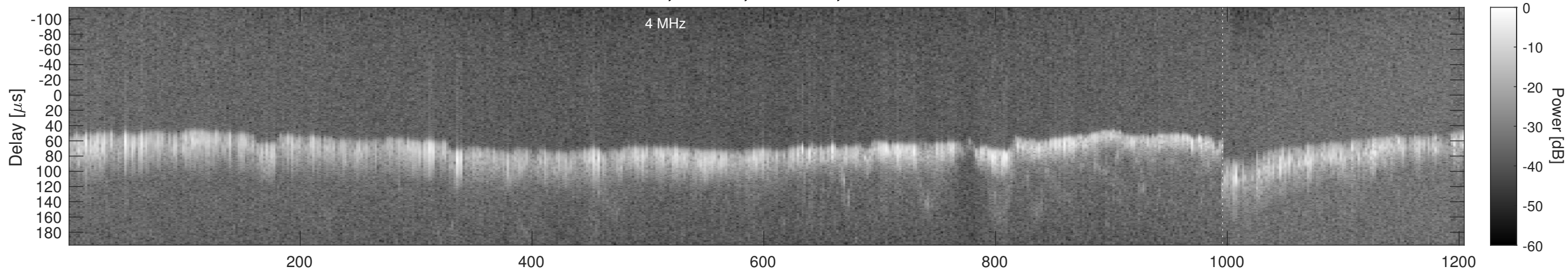
Orbit 4079, Window, Channel 2, Chapman
