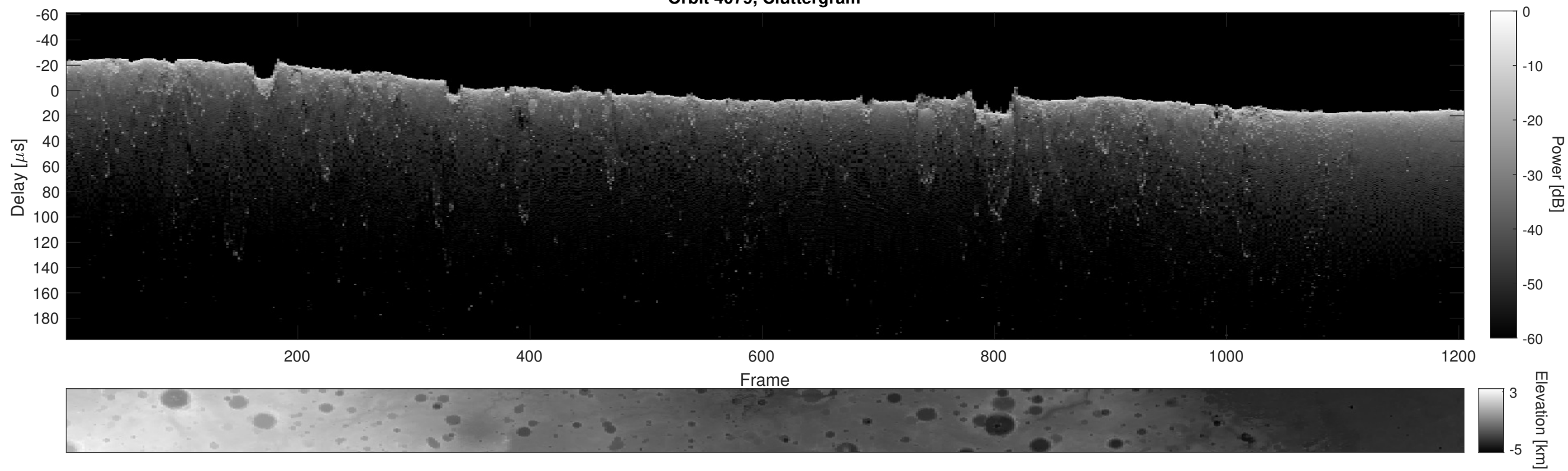
Orbit 4079, Cluttergram
