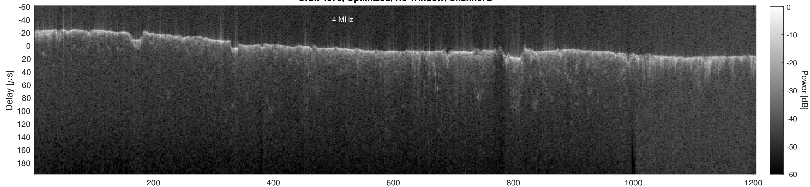
Orbit 4079, Cluttergram
