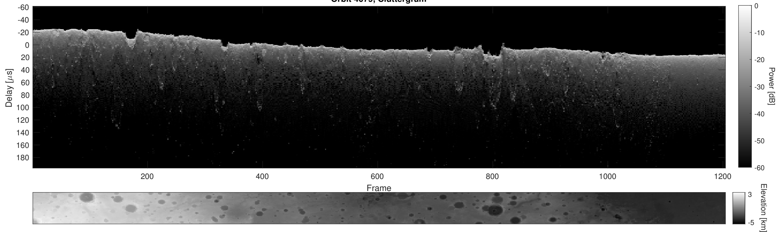
Orbit 4079, Cluttergram
