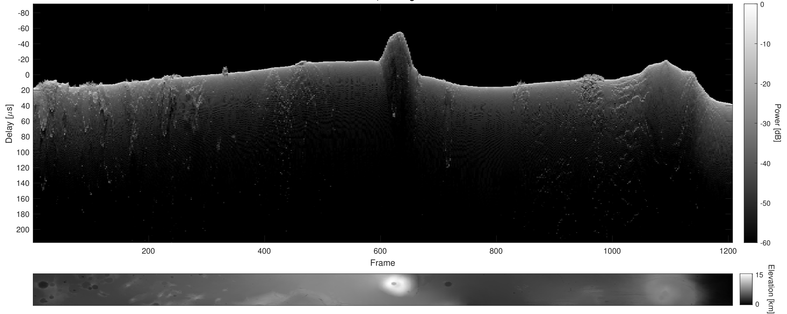
Orbit 4080, Cluttergram
