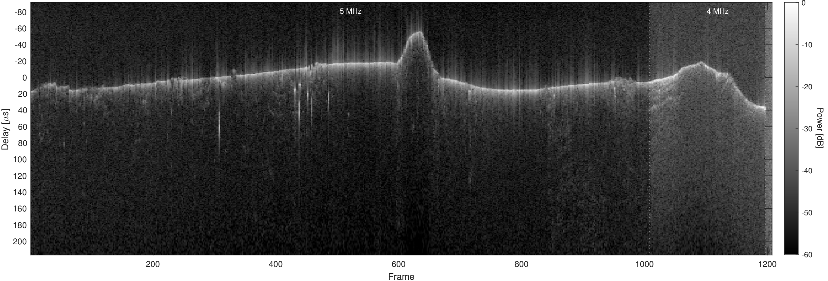
Orbit 4080, Optimized, No Window, Channel 2
