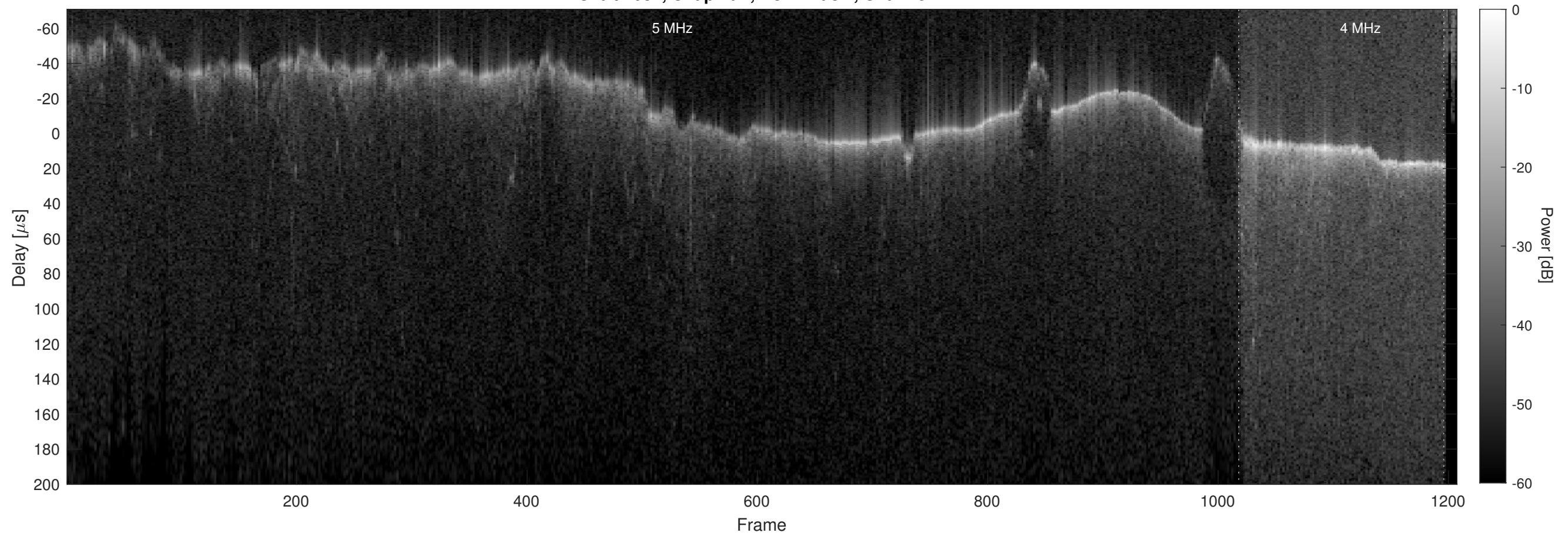
Orbit 4081, Chapman, No Window, Channel 2
