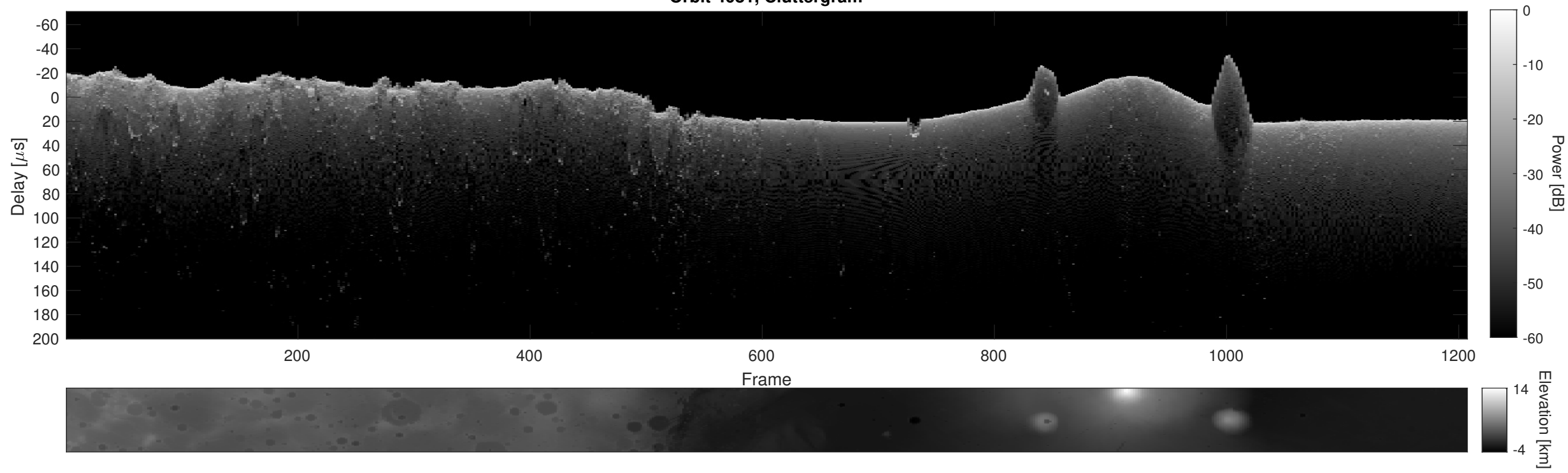
Orbit 4081, Cluttergram
