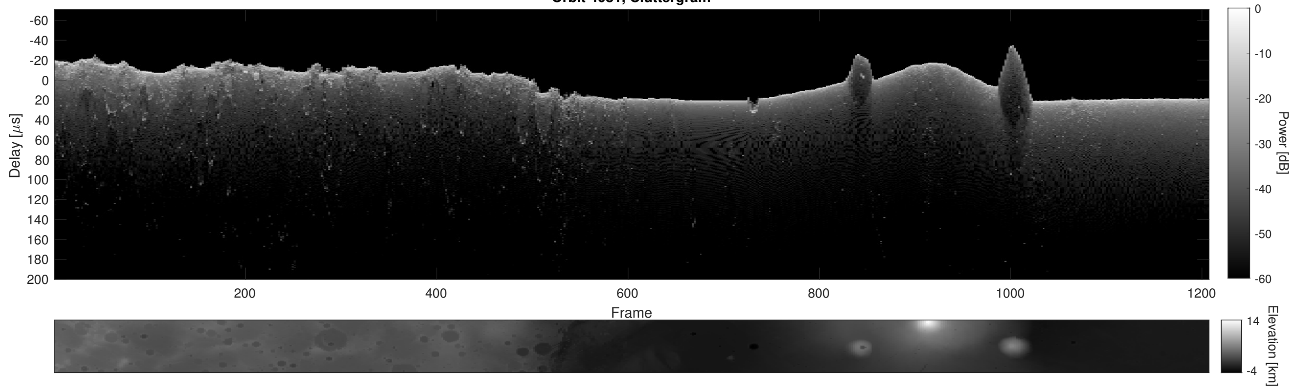
Orbit 4081, Cluttergram
