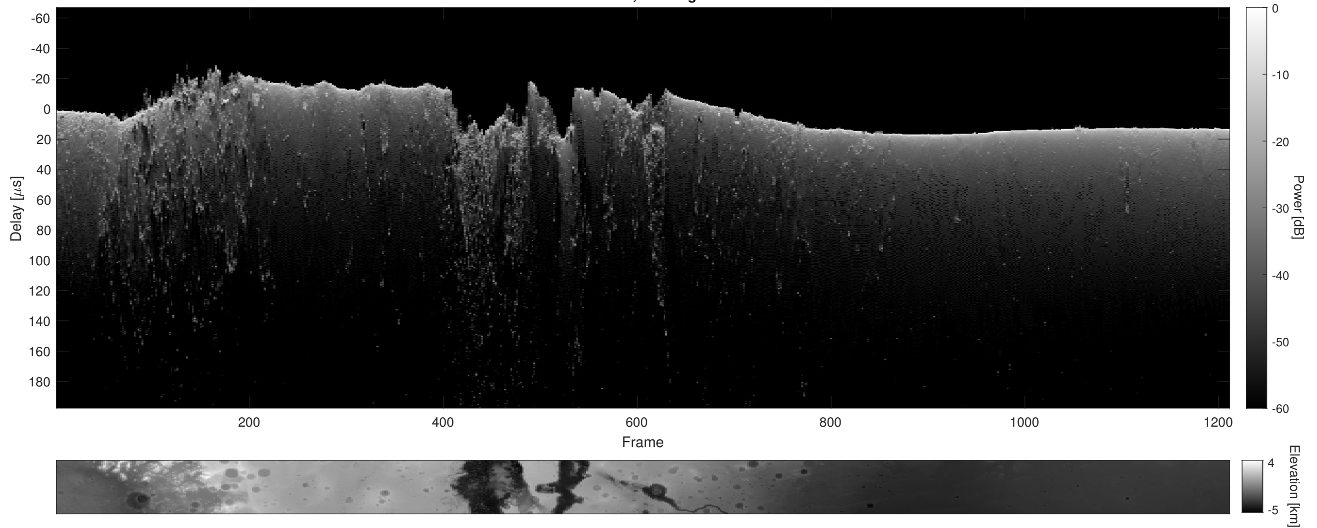
Orbit 4083, Cluttergram
