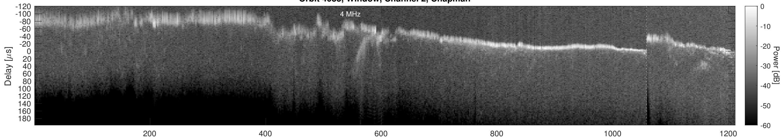
Orbit 4083, Window, Channel 2, Optimized
