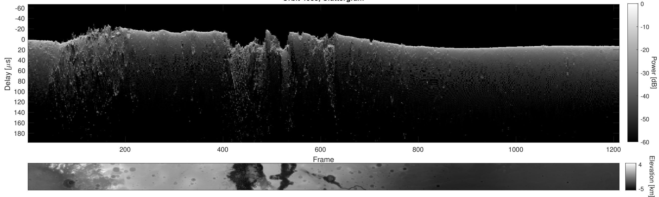
Orbit 4083, Cluttergram
