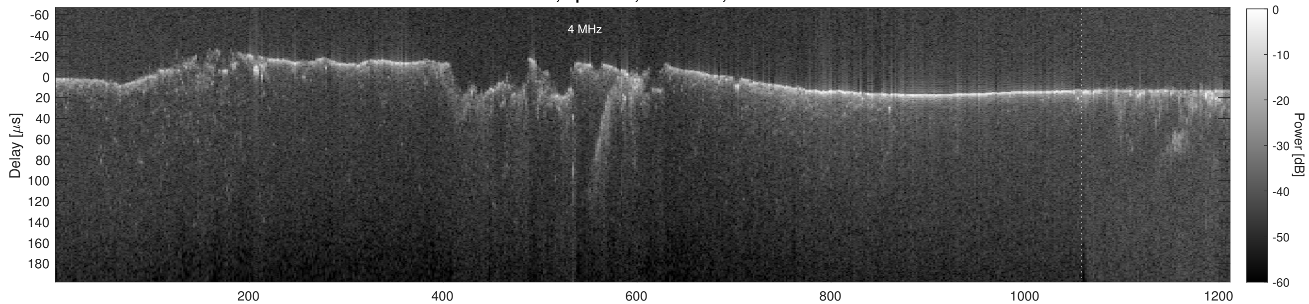
Orbit 4083, Cluttergram
