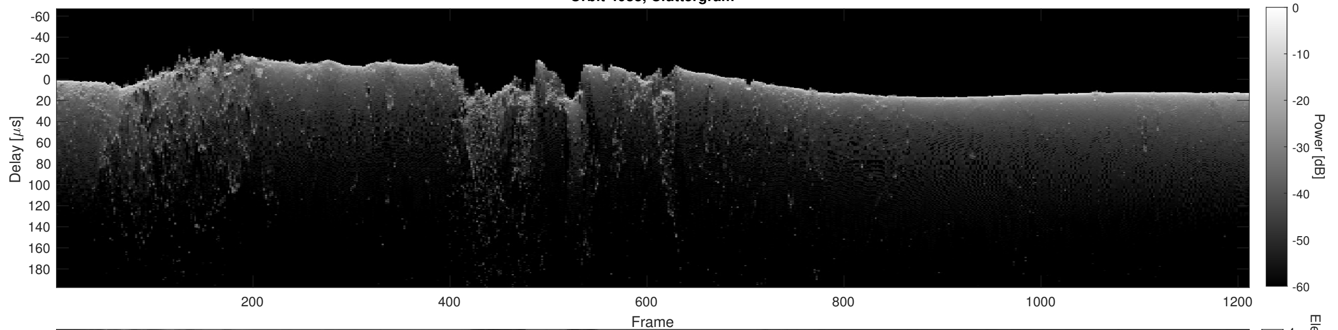
Orbit 4083, Cluttergram
