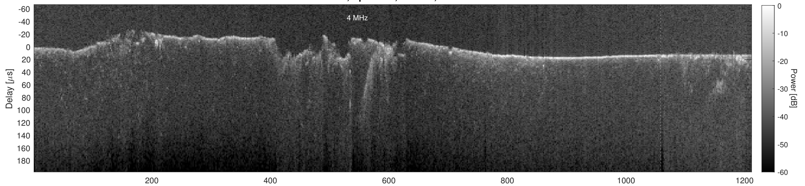
Orbit 4083, Cluttergram
