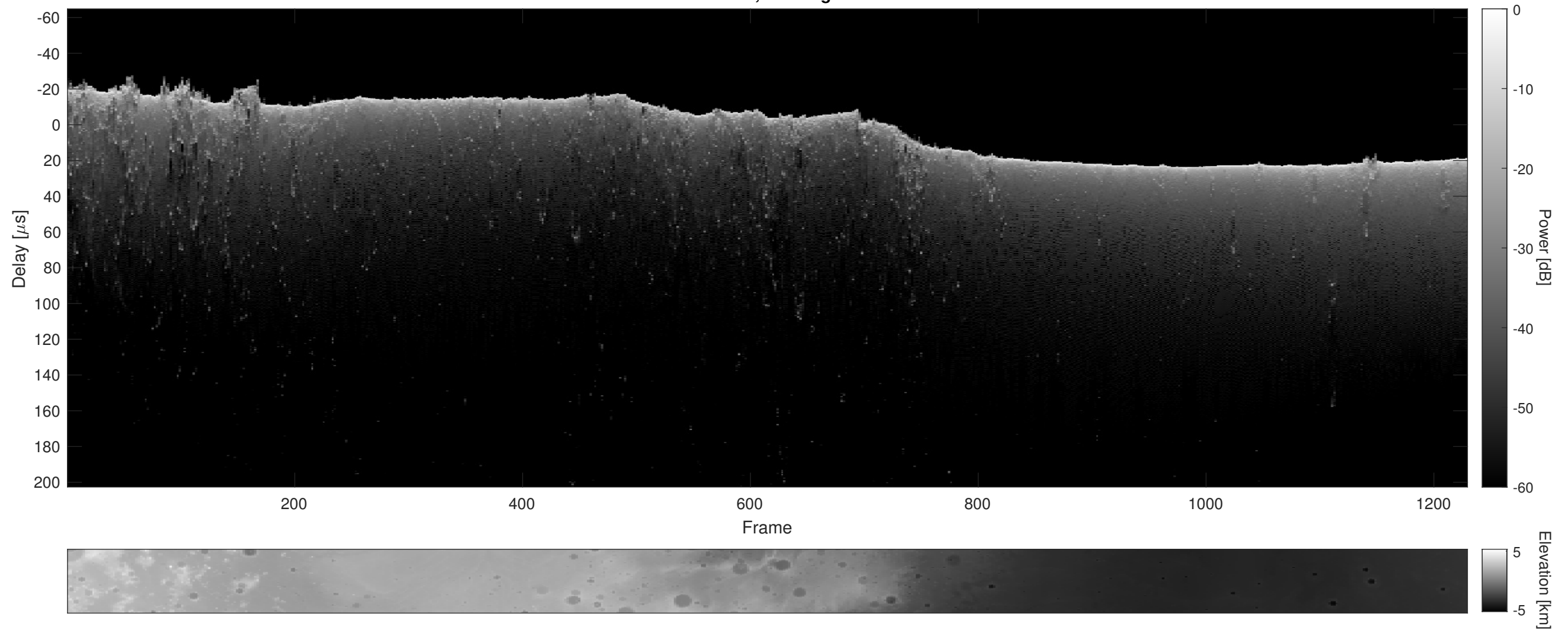
Orbit 4085, Cluttergram
