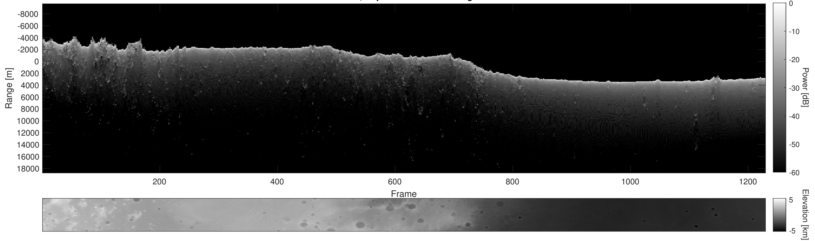
Orbit 4085, Depth-Corrected Cluttergram
