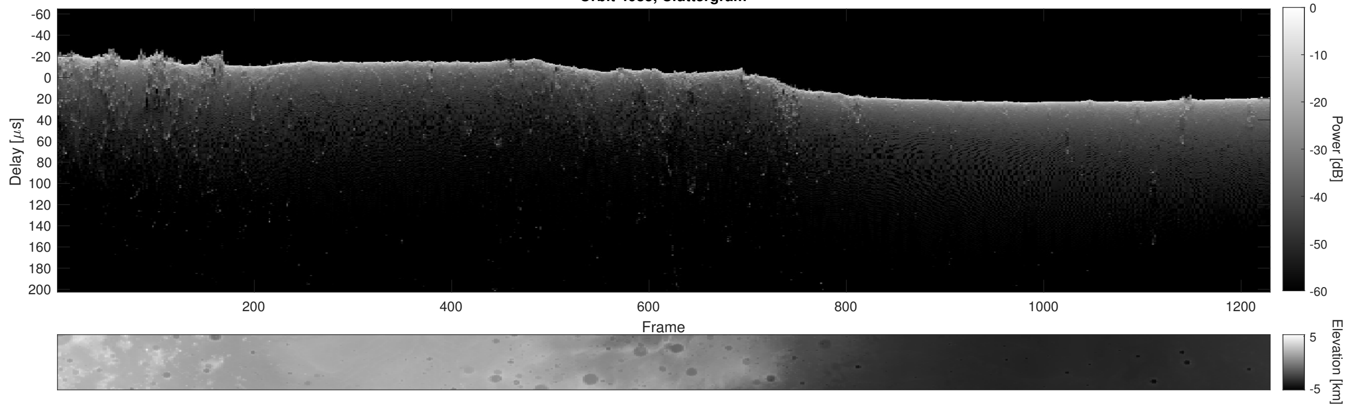
Orbit 4085, Cluttergram
