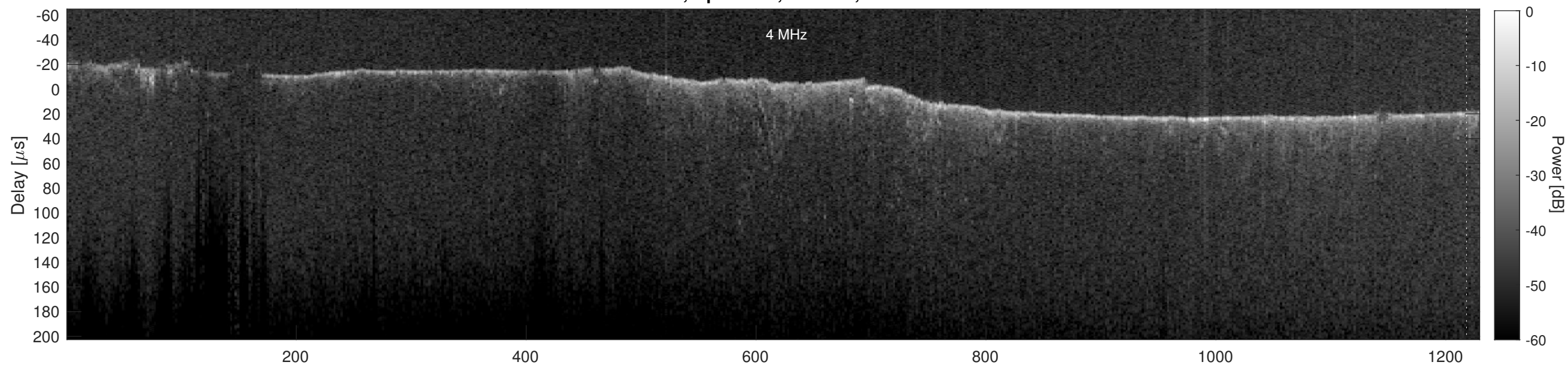
Orbit 4085, Cluttergram
