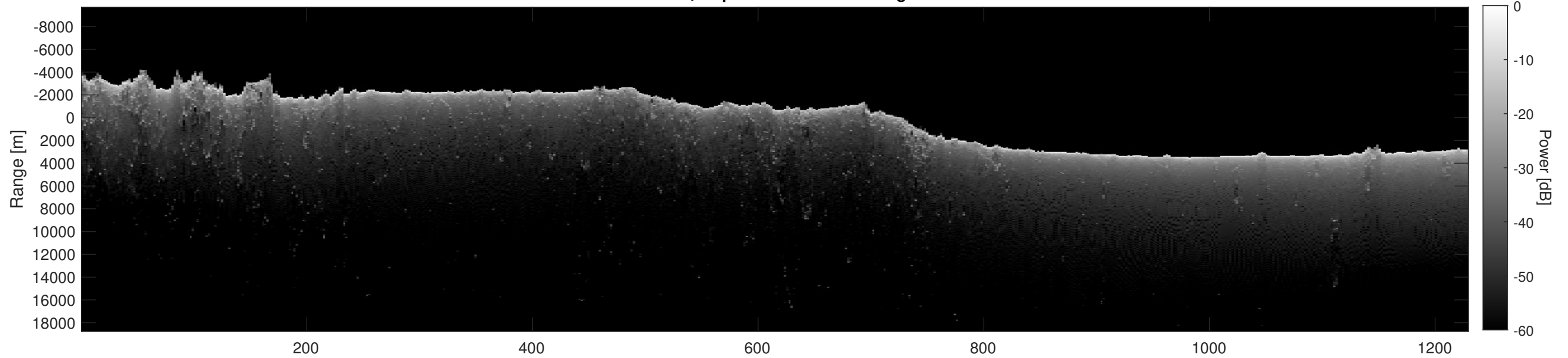
Orbit 4085, Depth-Corrected Cluttergram
