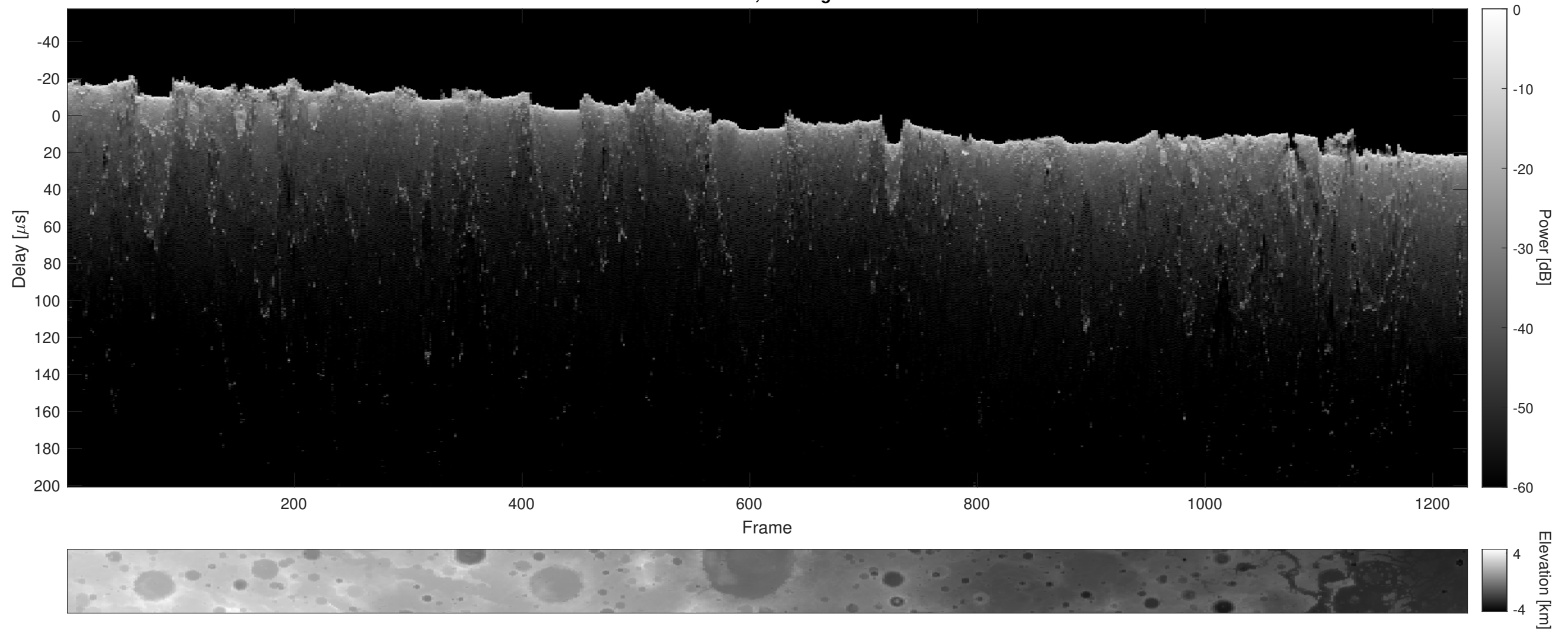
Orbit 4086, Cluttergram
