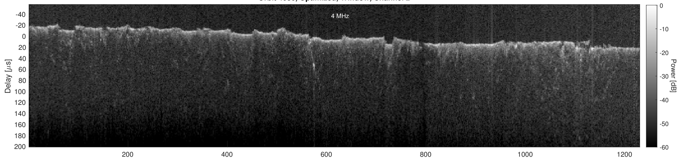
Orbit 4086, Cluttergram
