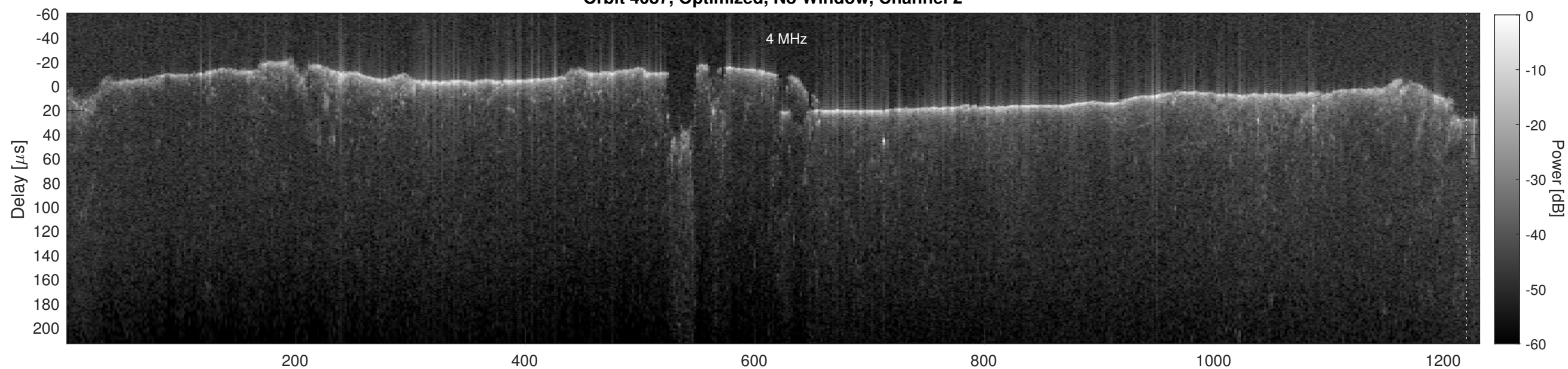
Orbit 4087, Cluttergram
