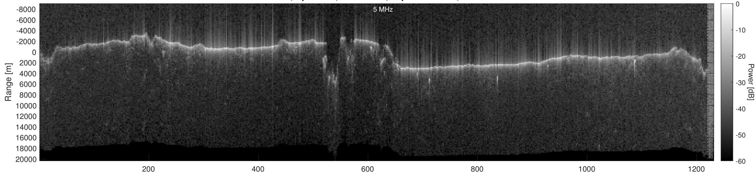
Orbit 4087, Optimized, No Window, Depth-Corrected, Channel 2
