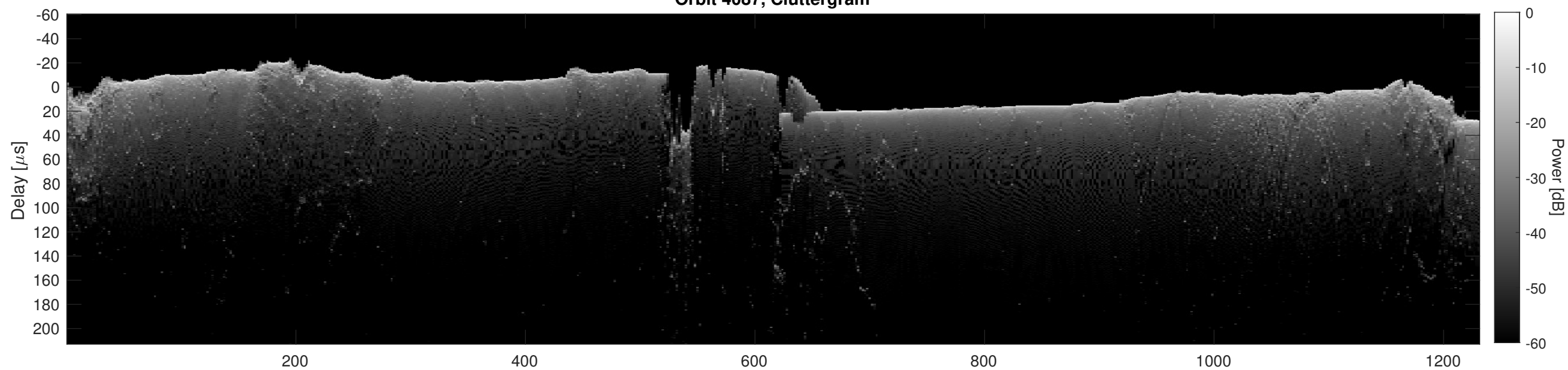
Orbit 4087, Cluttergram
