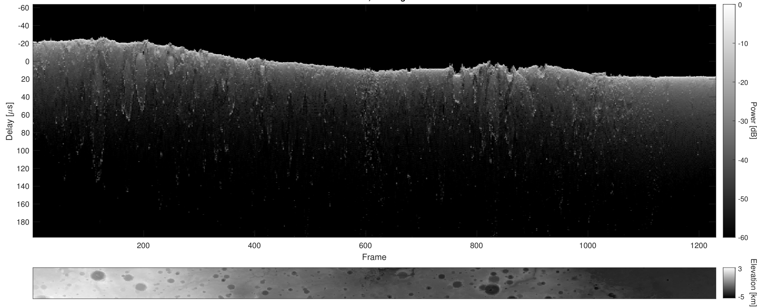
Orbit 4090, Cluttergram
