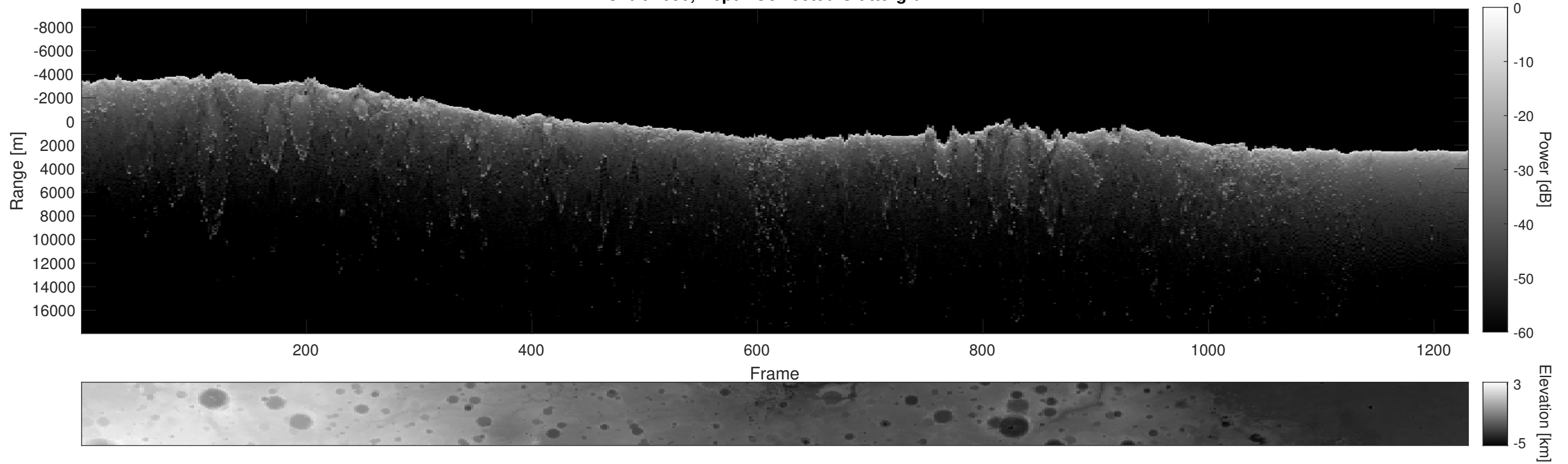
Orbit 4090, Depth-Corrected Cluttergram
