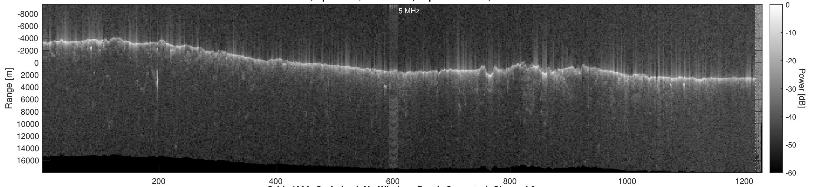
Orbit 4090, Optimized, No Window, Depth-Corrected, Channel 2
