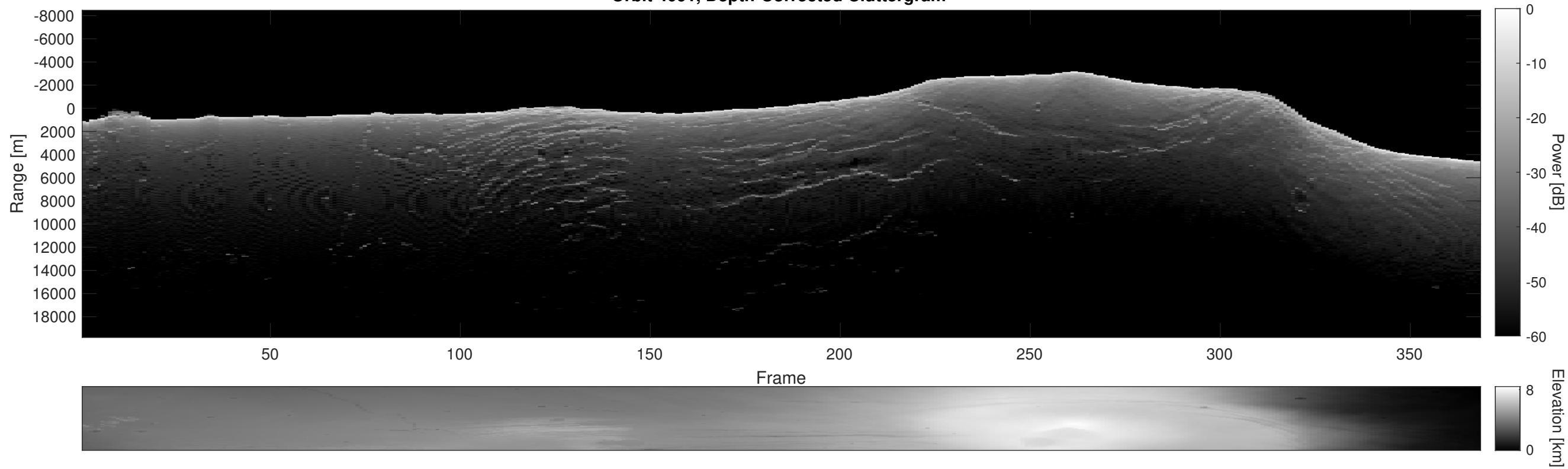
Orbit 4091, Depth-Corrected Cluttergram
