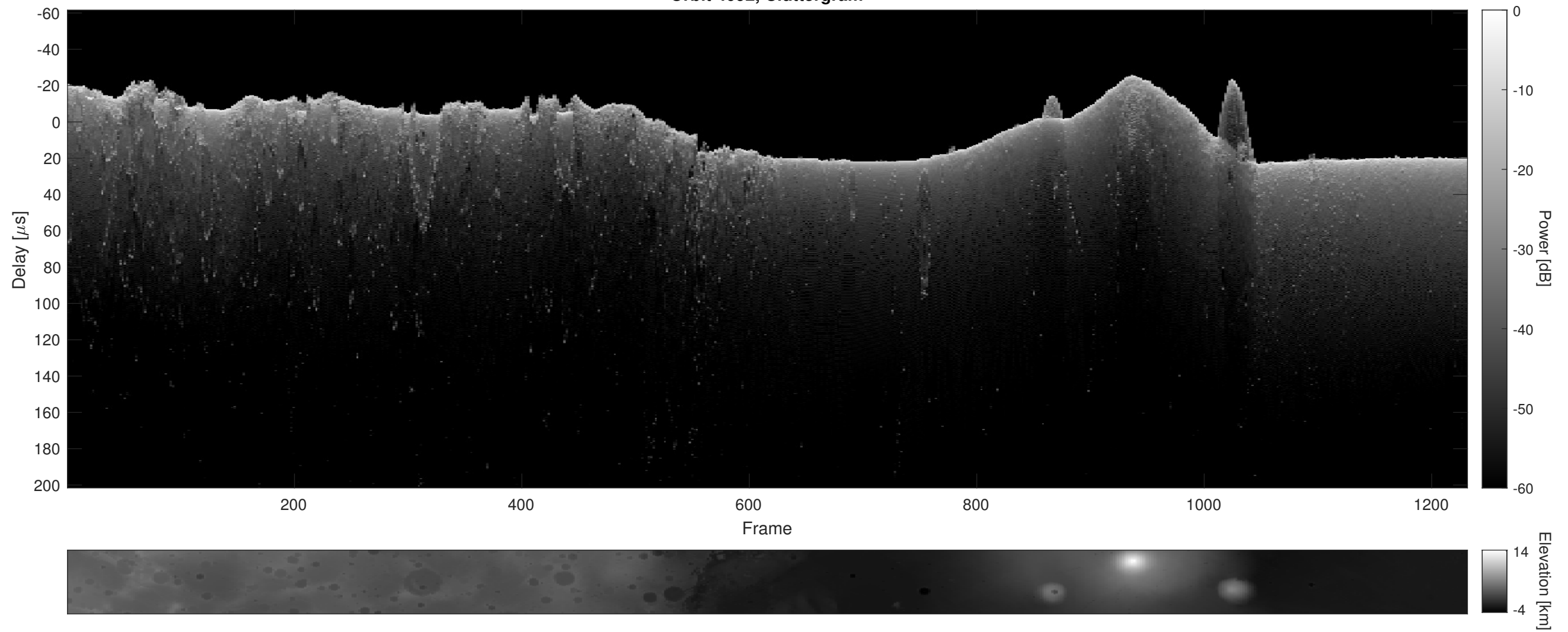
Orbit 4092, Cluttergram
