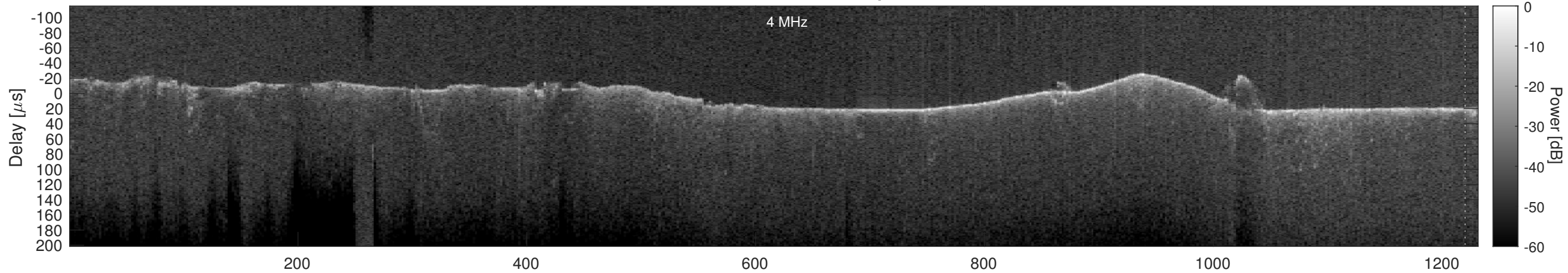
Orbit 4092, Cluttergram
