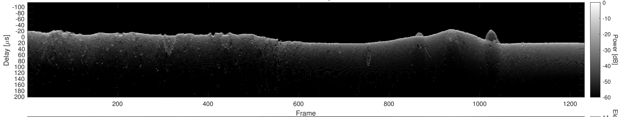
Orbit 4092, Cluttergram
