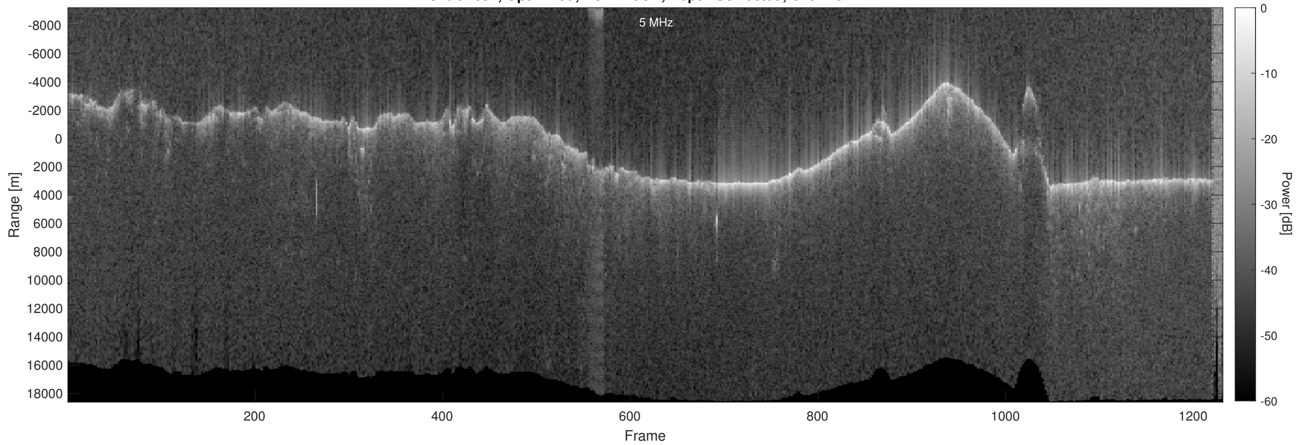
Orbit 4092, Optimized, No Window, Depth-Corrected, Channel 2
