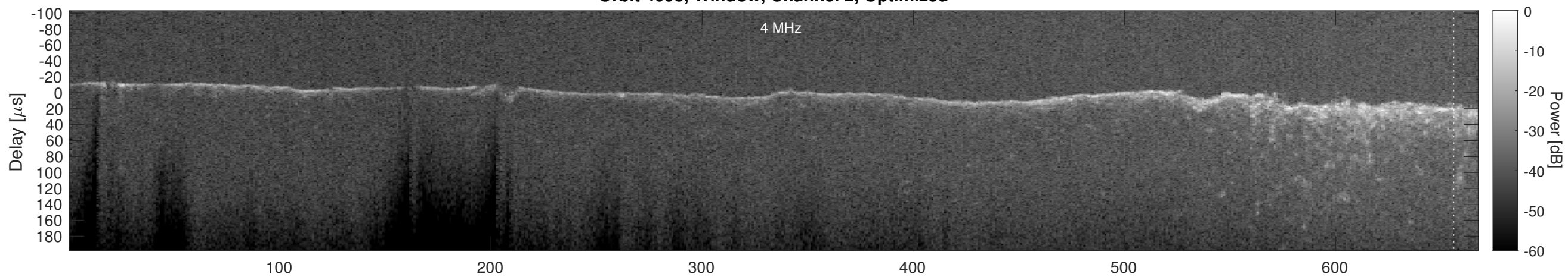
Orbit 4093, Cluttergram
