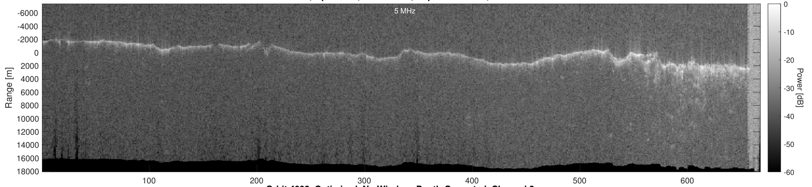
Orbit 4093, Optimized, No Window, Depth-Corrected, Channel 2
