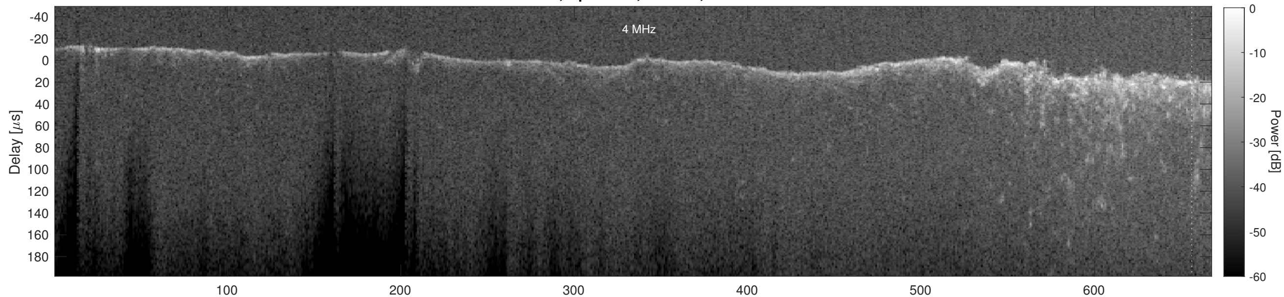
Orbit 4093, Cluttergram
