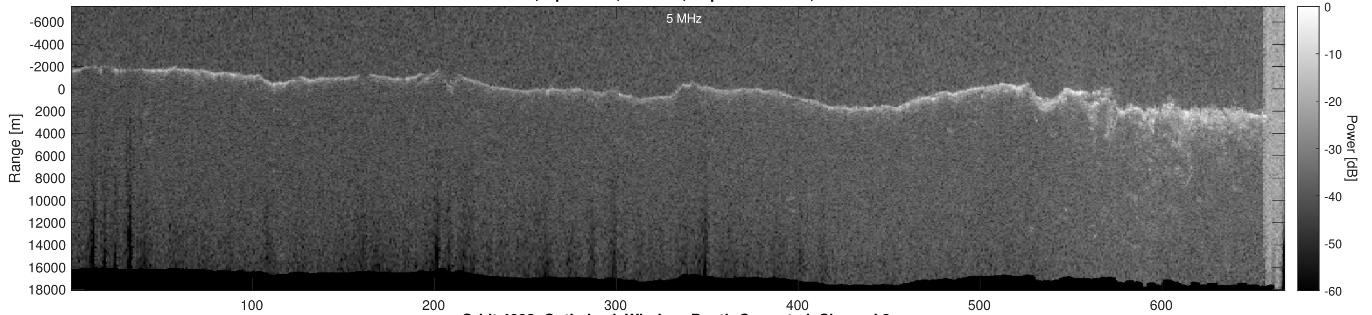
Orbit 4093, Optimized, Window, Depth-Corrected, Channel 2
