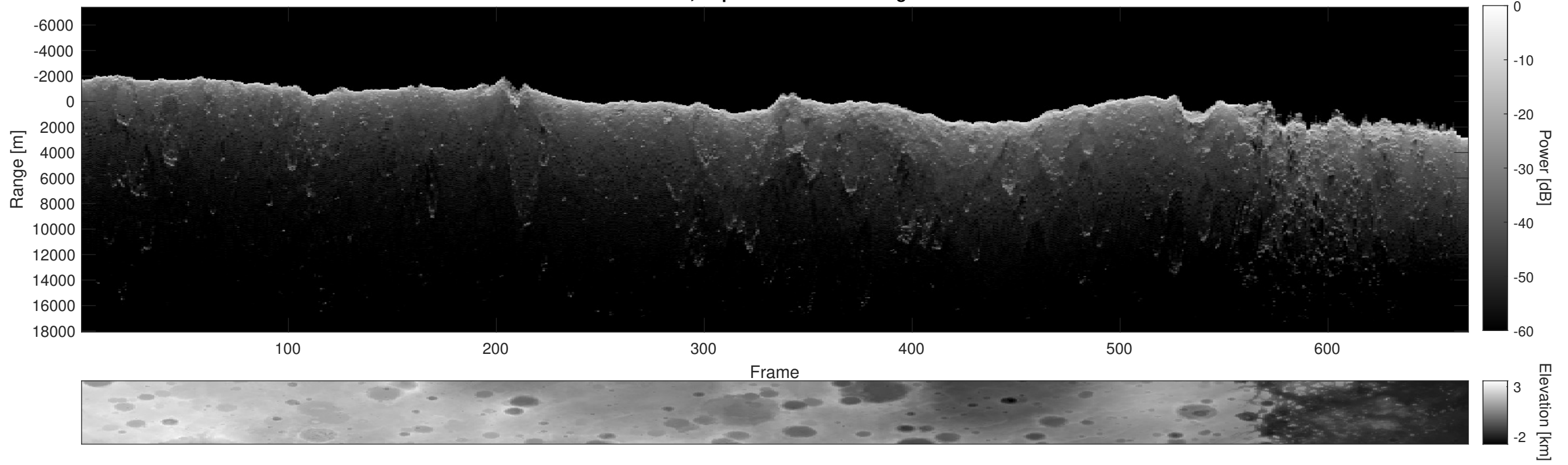
Orbit 4093, Depth-Corrected Cluttergram
