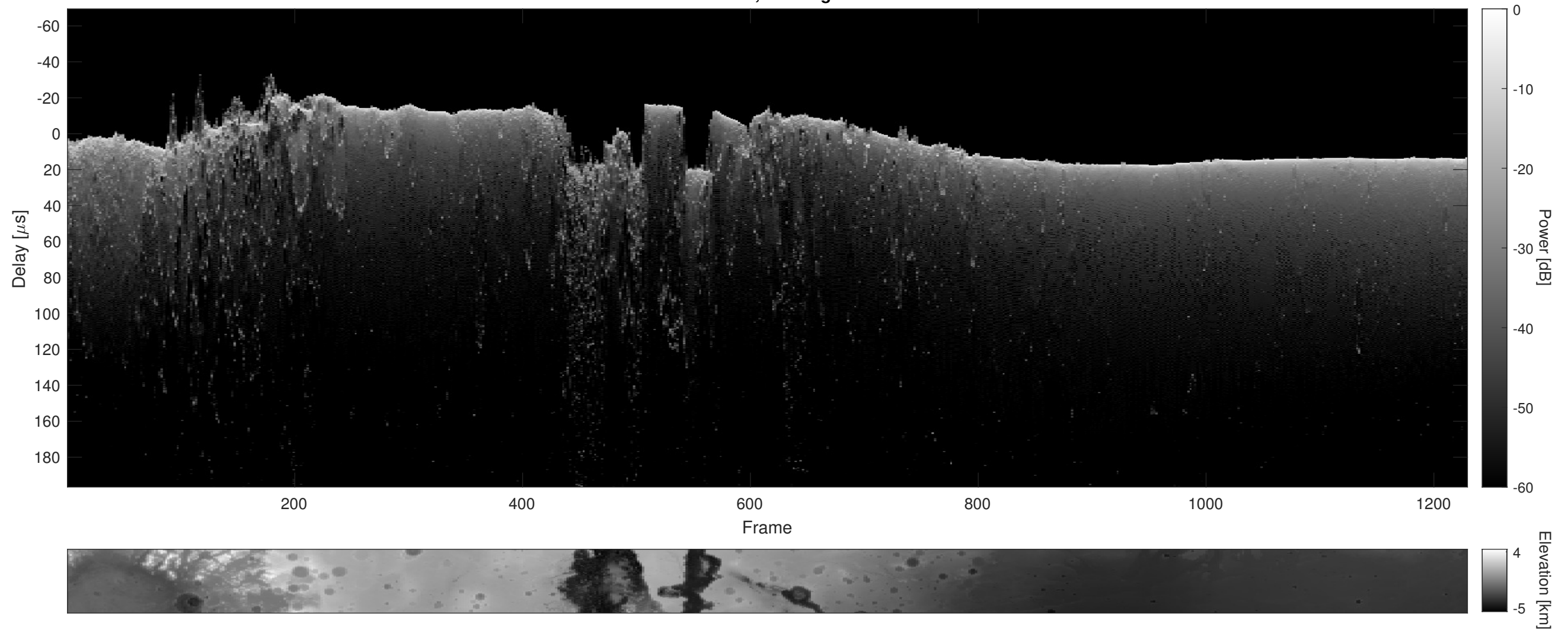
Orbit 4094, Cluttergram
