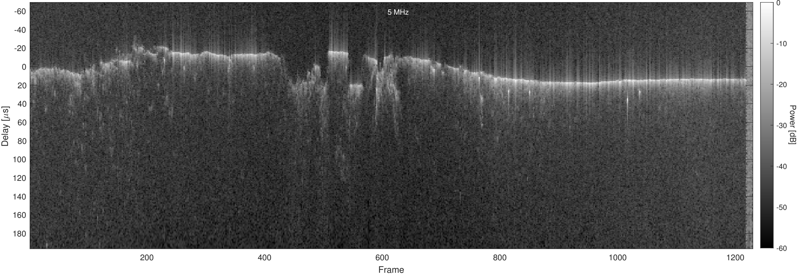
Orbit 4094, Optimized, No Window, Channel 2
