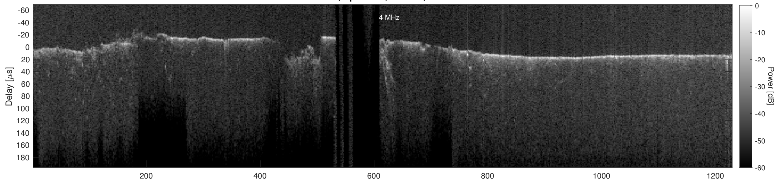
Orbit 4094, Cluttergram
