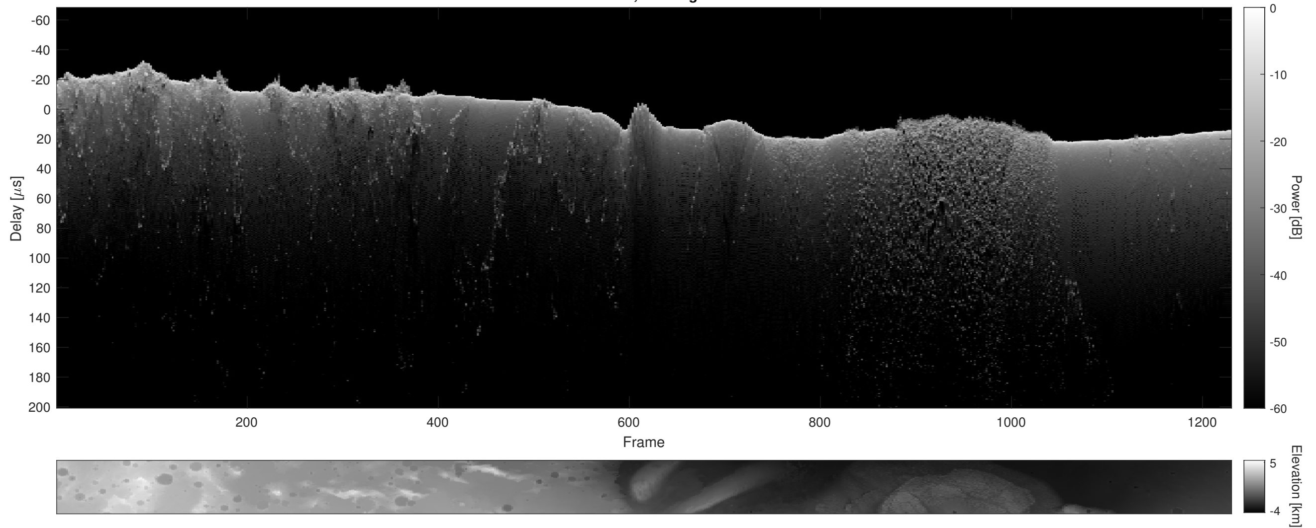
Orbit 4095, Cluttergram
