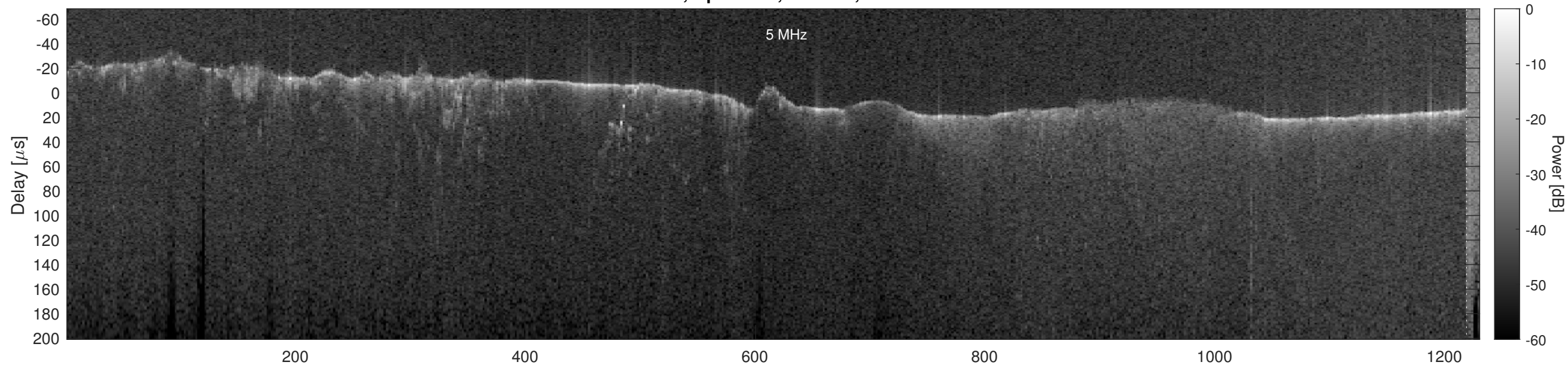
Orbit 4095, Optimized, Window, Channel 2
