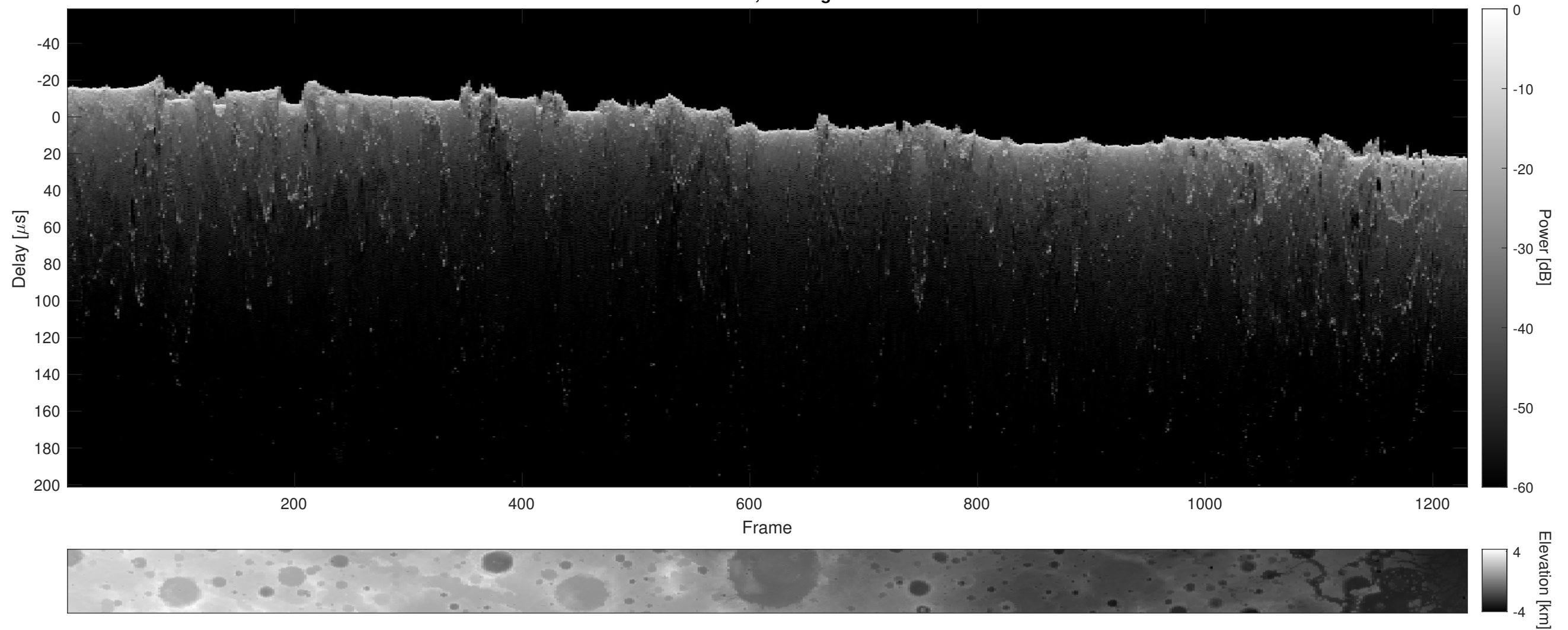
Orbit 4097, Cluttergram
