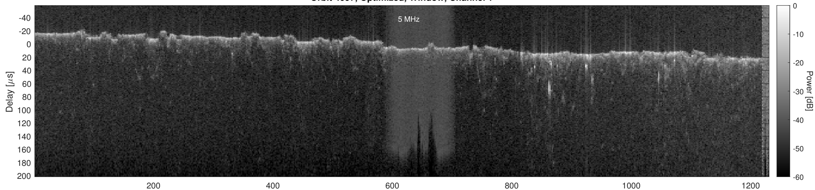
Orbit 4097, Optimized, Window, Channel 2
