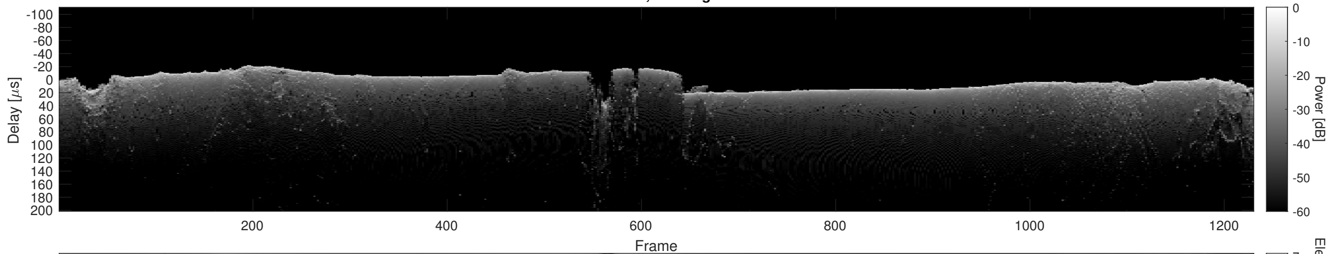
Orbit 4098, Cluttergram
