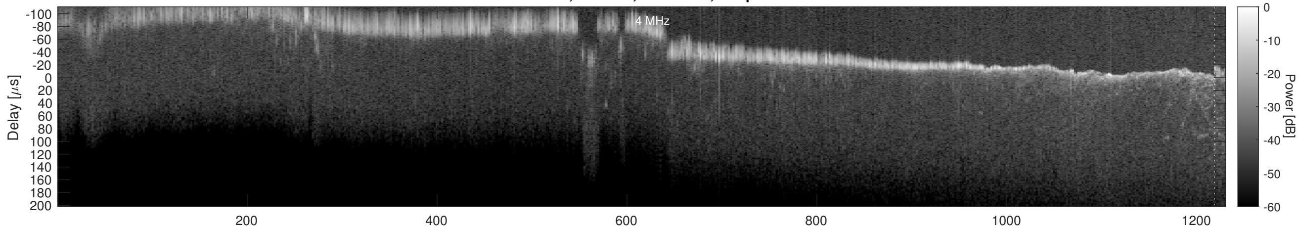
Orbit 4098, Window, Channel 2, Optimized
