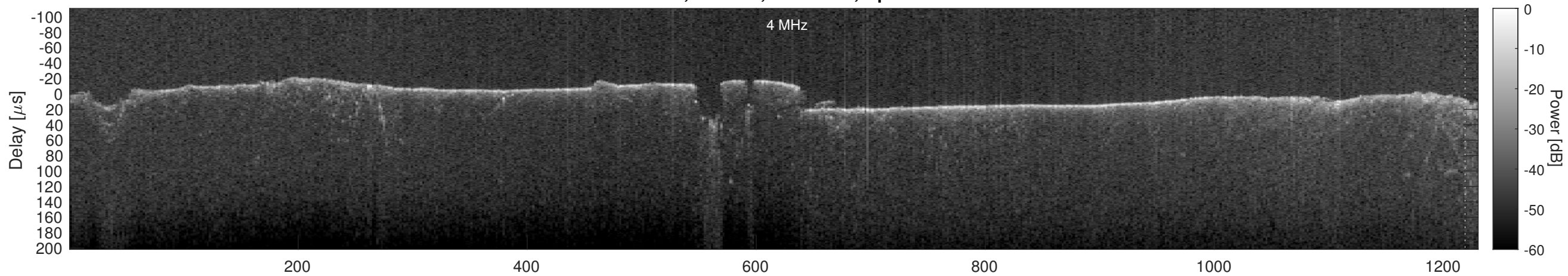
Orbit 4098, Cluttergram
