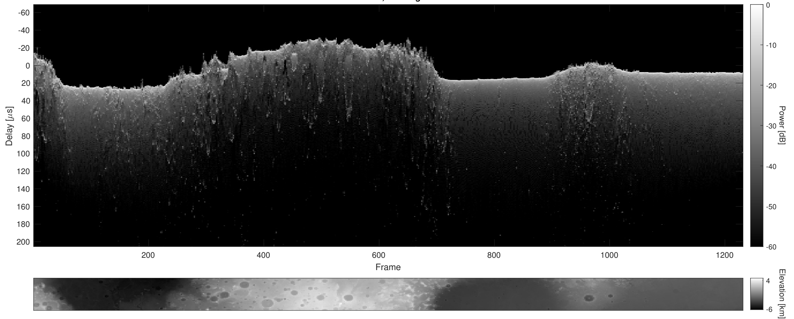
Orbit 4100, Cluttergram
