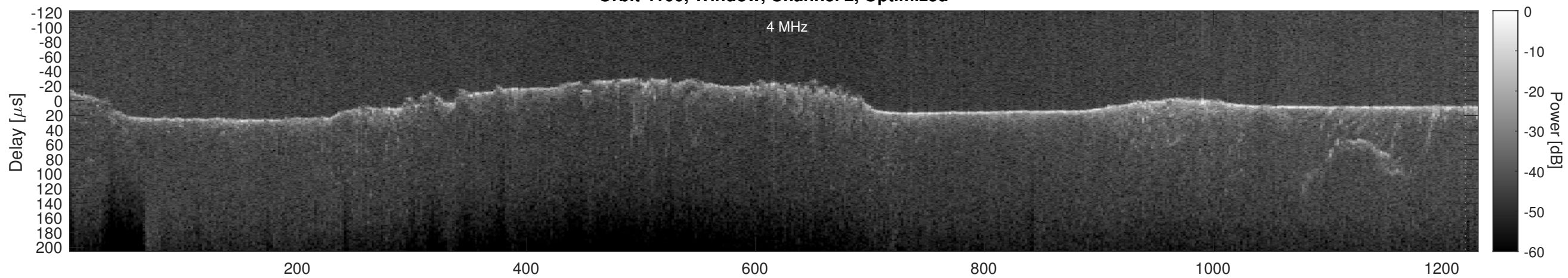
Orbit 4100, Cluttergram
