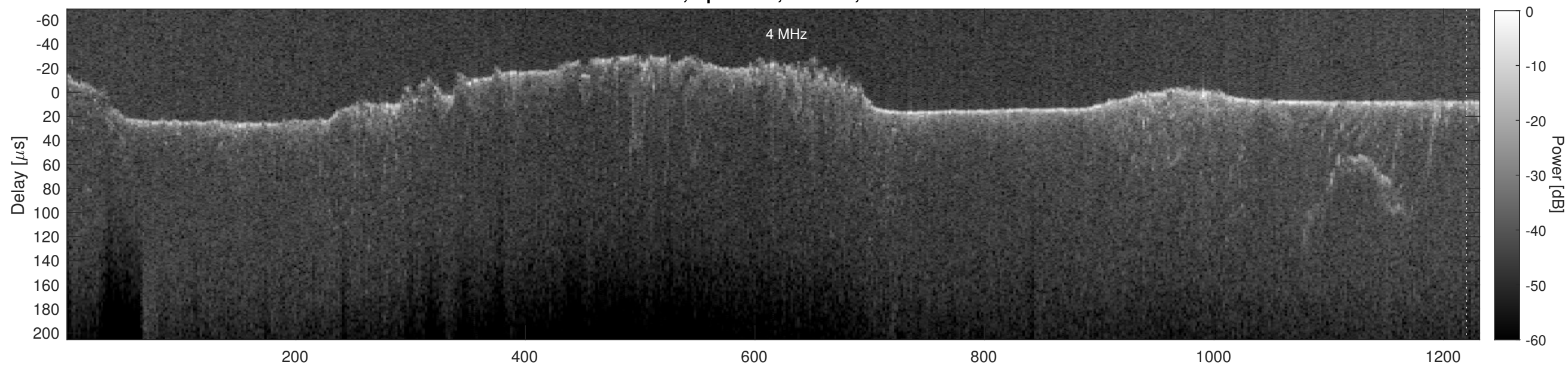
Orbit 4100, Cluttergram
