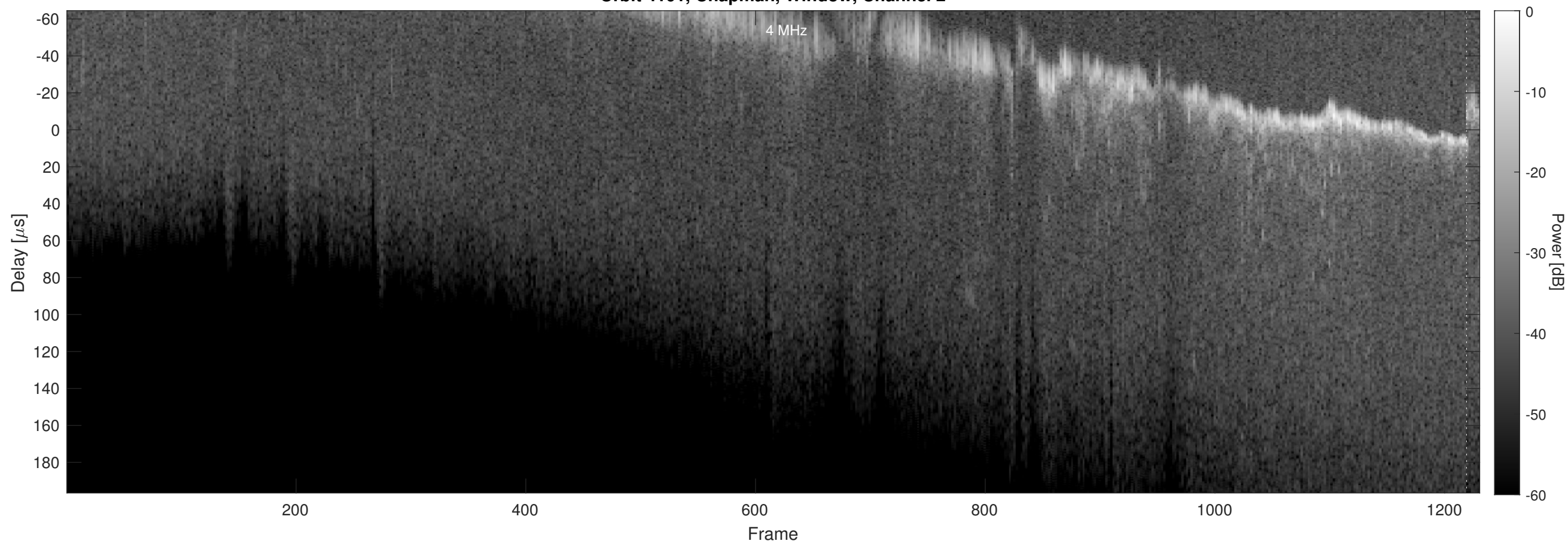
Orbit 4101, Chapman, Window, Channel 2
