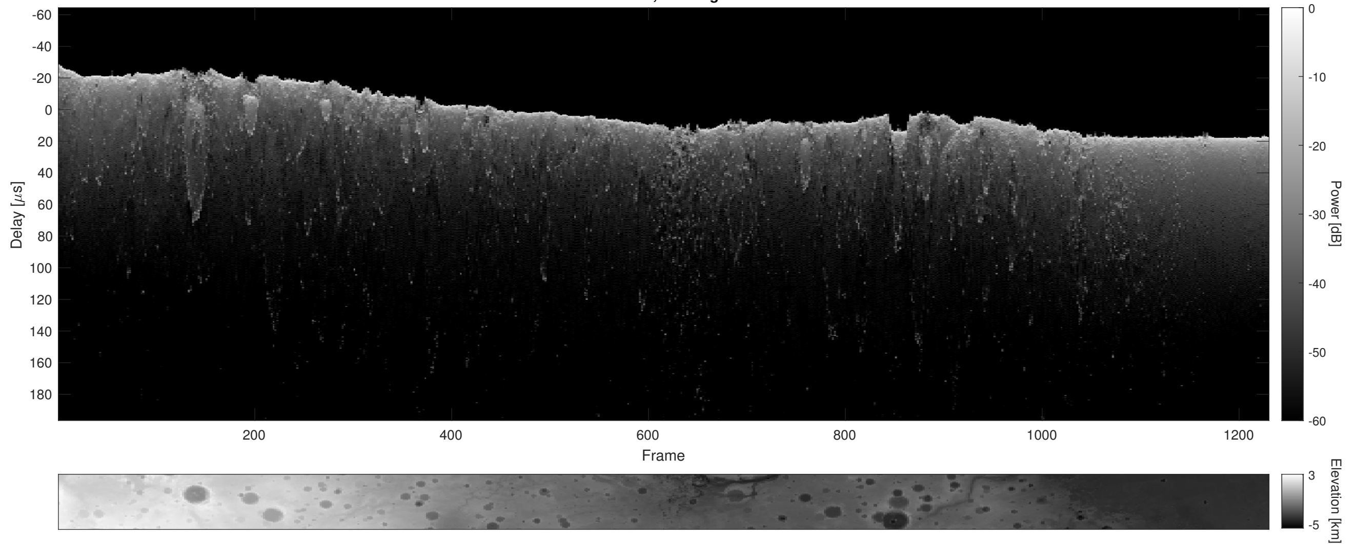
Orbit 4101, Cluttergram
