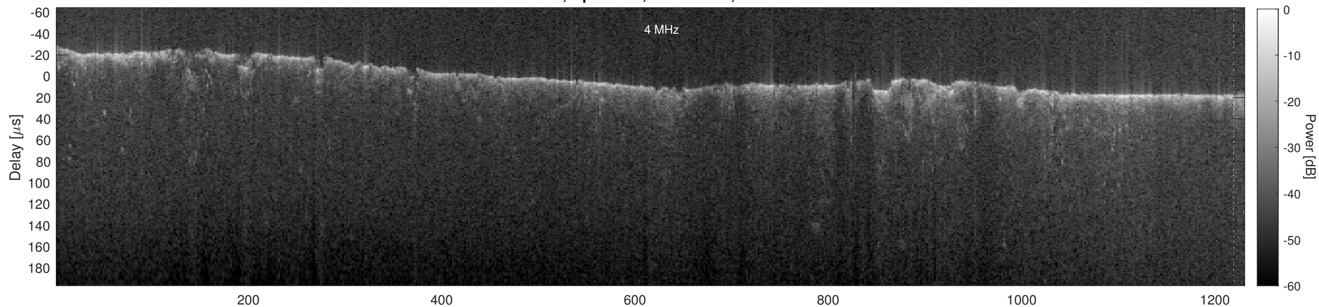
Orbit 4101, Cluttergram
