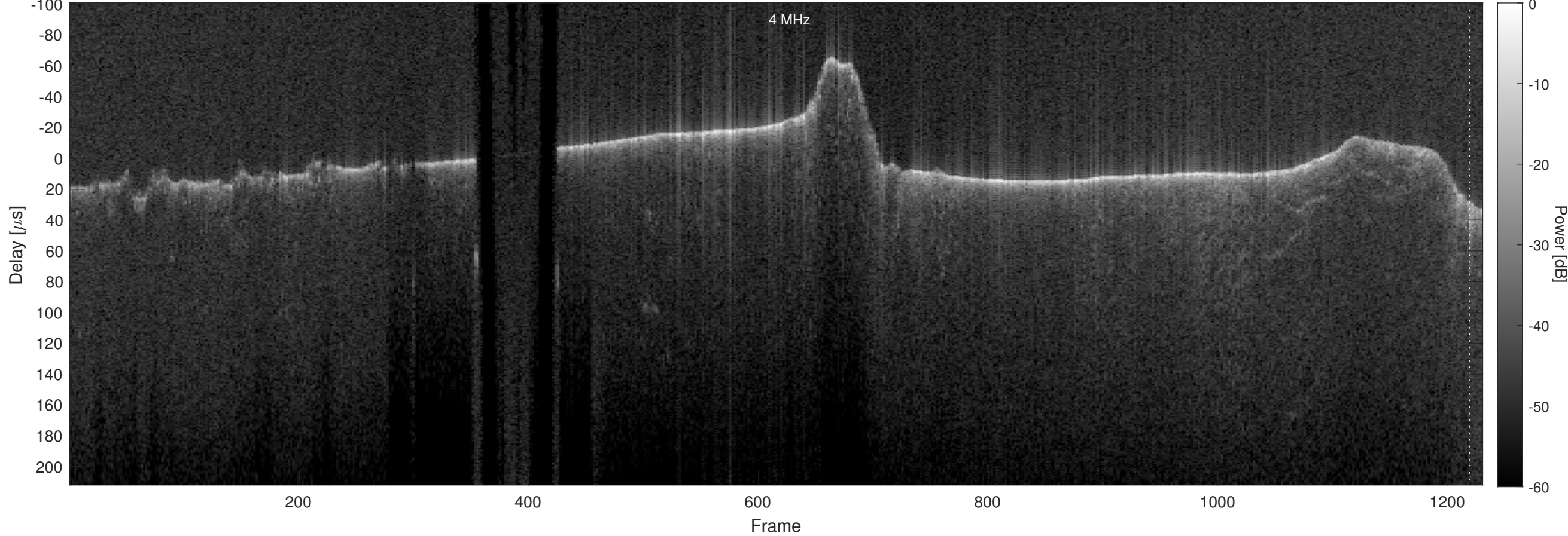
Orbit 4102, Optimized, No Window, Channel 2
